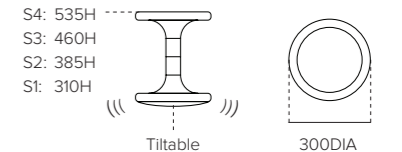
Dodo 300DIA Seat, with a Curved Base for Tilt Action Size 1: 310H / Size 2: 385H / Size 3: 460H / Size 4: 535H White Base and Black Seat with Red, Lime or Teal Ring
